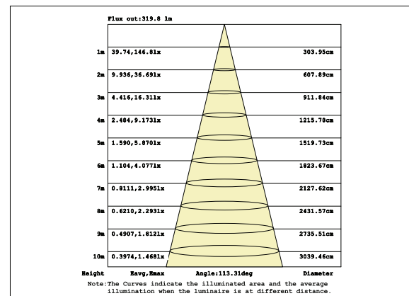
Illuminance curve
